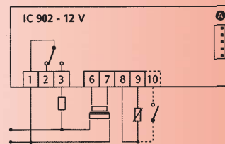
ID 902 PTC 12V
