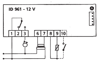
ID 961/A PTC
